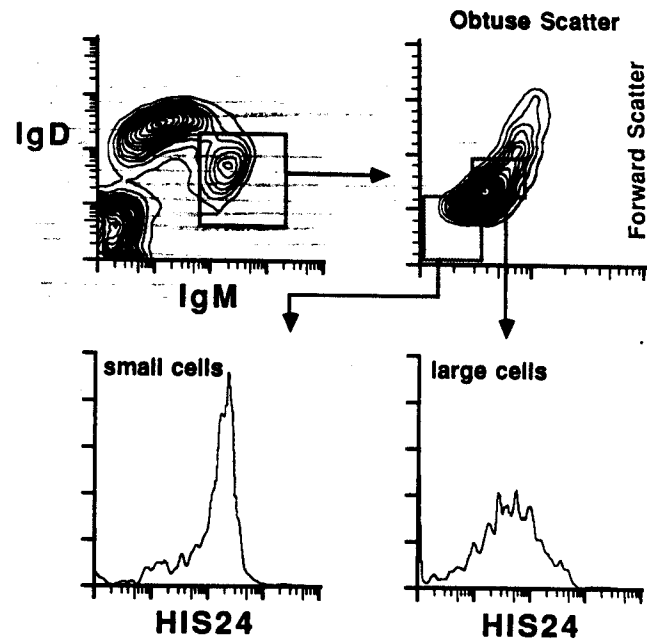
Figure 5. Three-color FCM analysis of rat spleen showing that relatively large population III cells ( IgM^{bright}IgD^{dull} ) are dull for HIS24, whereas the relatively small population III cells are bright for HIS24. Spleen cell suspensions were stained with fluoresceinated anti-rat IgM (HIS40), biotinylated anti-rat IgD (MARD 3) and APHC-HIS24. Texas red-avidin was used to reveal anti rat IgD.
