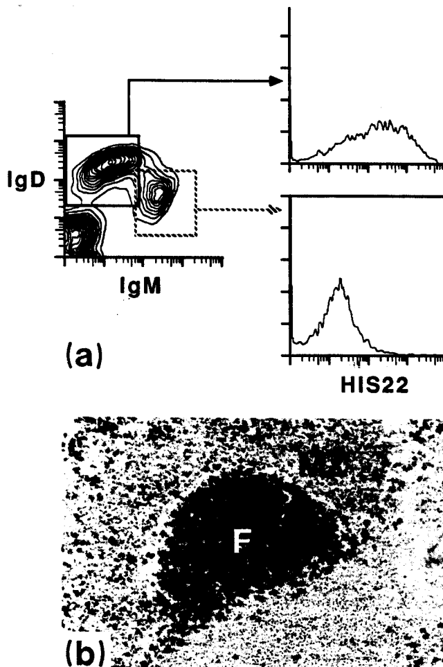
Figure 2. (a) Three-color immunofluorescence demonstrates that HIS22 mainly reacts with population I (IgM dull IgD bright ) cells; population III (IgM bright IgD dull ) cells and a minority of population I express only very low levels of the HIS22 determinant. Spleen cell suspensions were stained with fluoresceinated anti-rat IgM (HIS40), biotinylated anti-rat IgD (MARD 3) and APhC-HIS22. Biotin was revealed by Texas red-avidin. (b) In spleen sections, HIS22 reacts with B cells in lymphoid follicles (F); B cells located in the MZ are virtually unstained. Immunoperoxidase staining of a frozen section taken from a rat spleen. Note that in this follicle no GC is present (animals were not deliberately immunized; × 125).
