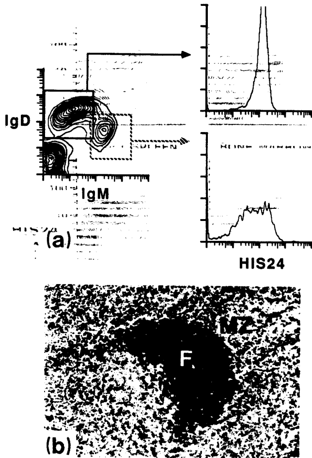
Figure 4. (a) Three-color immunofluorescence staining showing that HIS24 reacts brightly with virtually all population I ( IgM^{dull}IgD^{bright} ) cells and a small proportion of population III ( IgM^{bright}IgD^{dull} ) cells. About two thirds of population III cells express relatively low levels of the HIS24 determinant. Spleen cell suspensions were stained with FITC-anti-rat IgM (HIS40), biotinylated anti-rat IgD (MARD 3) and APHC-HIS24. Biotin was revealed by Texas red-avidin. (b) In spleen sections B cells expressing high levels of the HIS24 determinant are mainly found in lymphoid follicles (F) but not in MZ. Frozen section of rat spleen stained by immunoperoxidase with HIS24. Note that no GC is seen in this follicle. ( \times 125 ).
