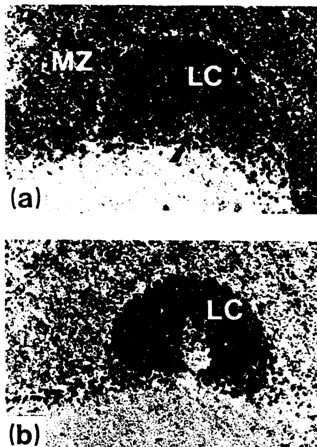
Figure 7. Reactivity patterns of serial sections from rat spleen with anti-IgM (a) and anti-IgD (b) showing that cells located in the lymphocyte corona (LC) of the lymphoid follicles express IgM and IgD, whereas MZ B cells express IgM but only very low levels of IgD. Note the presence of a very small (IgD - ) GC (arrow) in the follicle. Frozen sections of rat spleen (same animal as in Figs. 2 and 4) were stained by immunoperoxidase using anti-rat IgM (HIS40) or anti-rat IgD (MARD 3). (× 125).
